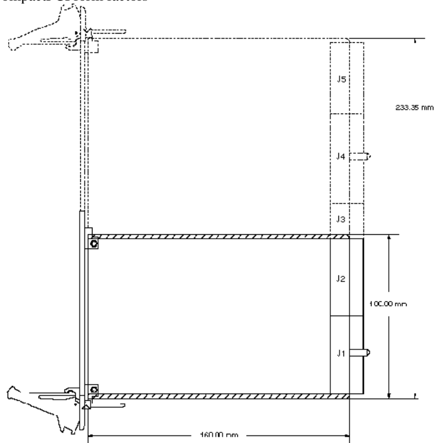
Figure 1. CompactPCI form factors
