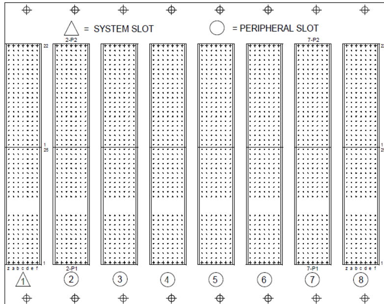
Figure 2. 3U CompactPCI Backplane.
